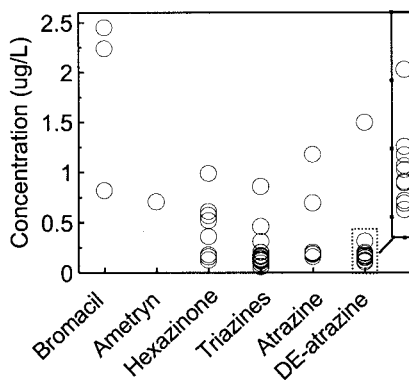
Figure 3. Herbicides and their degradates detected in wells in Hawaii sampled from September 1997 to January 1998.
